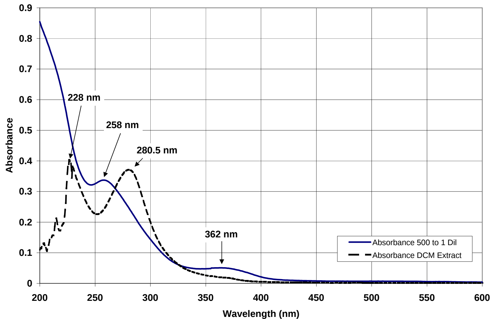
UV/Vis Spectrum of POM Brand Pomegranate Juice
